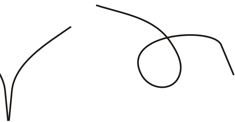
Varieties with singularities
