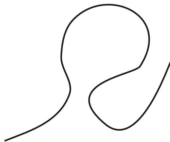
Variety without singularities
